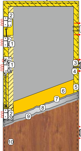
KMT Plus 75 passive
