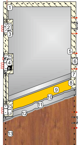
KMT Classic RC 3
